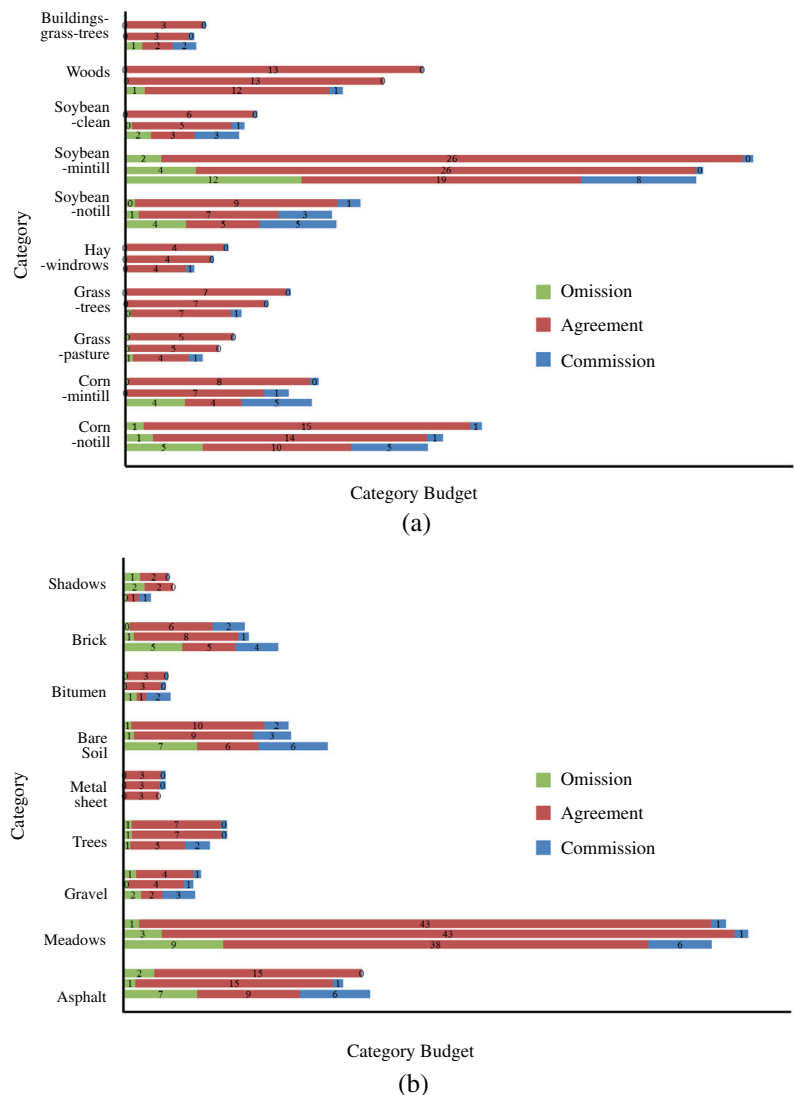
Fig. 7. Classification omission, agreement, and commission for each category over the three classifiers. For each class, the upper bar in the set is for NJCRC-KE, the middle bar is associated with NJCRC-KC, and the bottom one refers to CRC. Furthermore, the number in each bar is the associated proportion of the whole test dataset. (a) The Indian Pines image, and (b) the Pavia University image.
