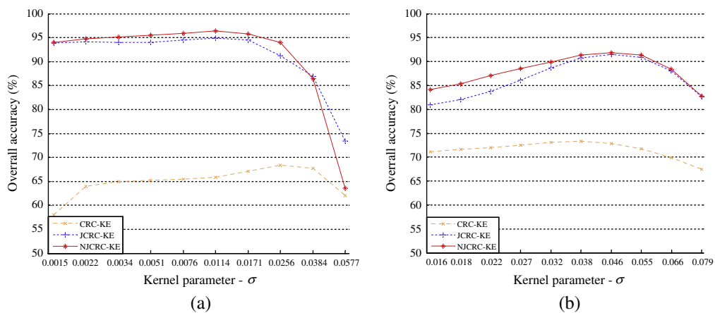
Fig. 6. The classification accuracy versus the kernel width parameter \sigma for the various classification algorithms: (a) the Indian Pines image; (b) the Pavia University image.
